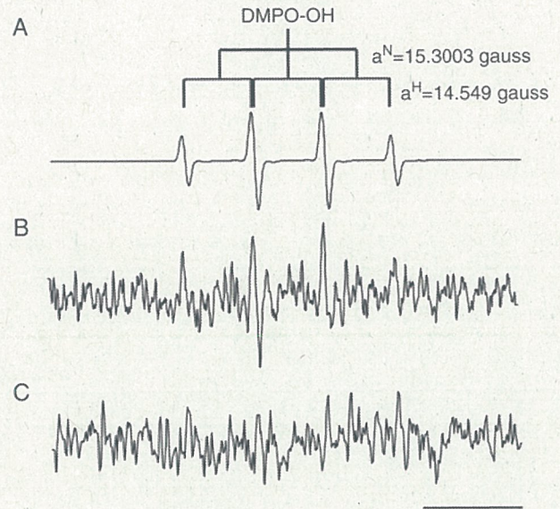
Figure 5. EPR spectrum in E. coli exposed to H_2O_2 and L-histidine. (A) Authentic spectrum of standard DMPO-OH. (B) EPR spectrum in E. coli exposed to 100 mM H_2O_2 and 100 mM L-histidine. (C) EPR spectrum in E. coli following exposure to 100 mM H_2O_2 alone. The bar indicates 20 gauss. EPR, electron paramagnetic resonance; DMPO, 5,5-dimethyl-1-pyrroline-N-oxide.
