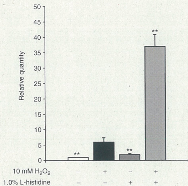
Figure 2. Relative quantification of recA gene expression in E. coli following exposure to hydrogen peroxide with L-histidine. The E. coli strain MG1665, grown to mid-logarithmic phase under aerobic conditions, was incubated in distilled water, 10 mM hydrogen peroxide, 1% L-histidine, or 10 mM hydrogen peroxide plus 1% L-histidine for 30 min at 37°C. The expression of recA relative to the distilled water treatment following exposure to the test reagents are shown. Samples are indicated as follows: H 2 O, open column; H 2 O 2 , closed column; L-histidine, gray column; and H 2 O 2 /L-histidine combination, hatched column. Data are expressed as the mean ± standard deviation of three independent repeats. **P<0.01 vs. H 2 O 2 alone.
